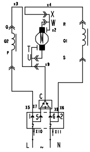
Electric Circuit
